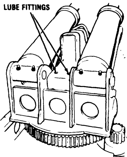
LOWER TENSION LINK PIVOT
