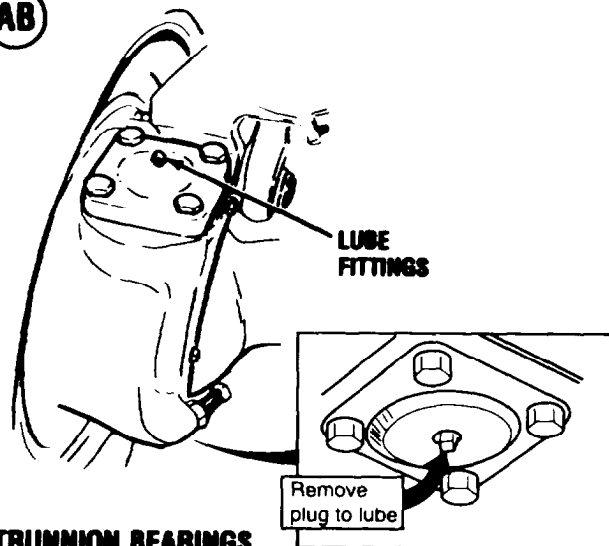
TRUNION BEARINGS (Right Side)
