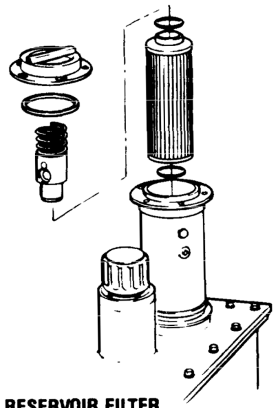
HYDRAULIC RESERVOIR FILTER
