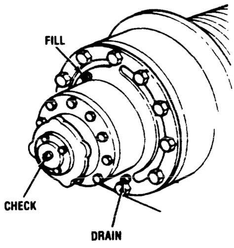
HEAVY-DUTY WINCH
