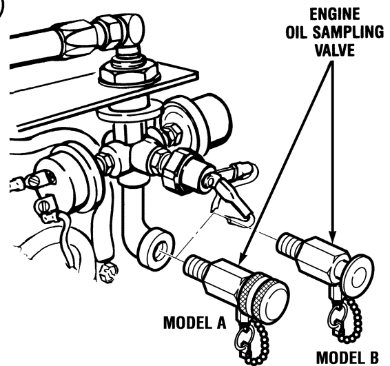
ENGINE OIL SAMPLING VALVE
